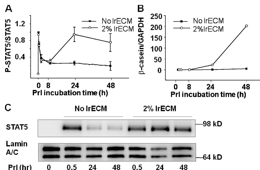
Figure 3. \beta -Casein transcription corresponds with IrECM-induced sustained STAT5 activation. (A) Eph4 cells on polyHEMA were treated with Prl alone or Prl plus 2% IrECM for different intervals. STAT5 phosphorylation was detected by Western blotting. The Western blot results were quantified by AlphaEaseFC software and expressed as relative levels of phosphorylated STAT5 to total STAT5 ( n = 3 ). (B) Quantification of \beta -casein mRNA levels by real-time RT-PCR. Eph4 cells on polyHEMA were treated with Prl alone or Prl plus 2% IrECM for different time points before RNA extraction. (C) Western blot analysis of nuclear levels of STAT5 in Eph4 cells. Cells on polyHEMA were treated with Prl alone or Prl plus 2% IrECM for 30 min or 24 or 48 h.
