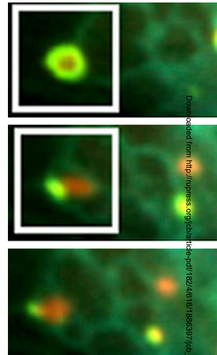
A newborn autophagosome (red) emerges from an omegasome (green circle).
