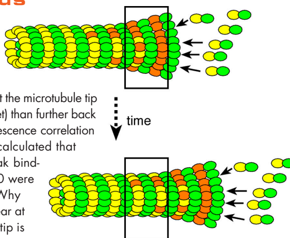
Binding sites (orange) for CLIP-170 are abundant at microtubule plus ends (top) but disappear as the filament grows (bottom).
