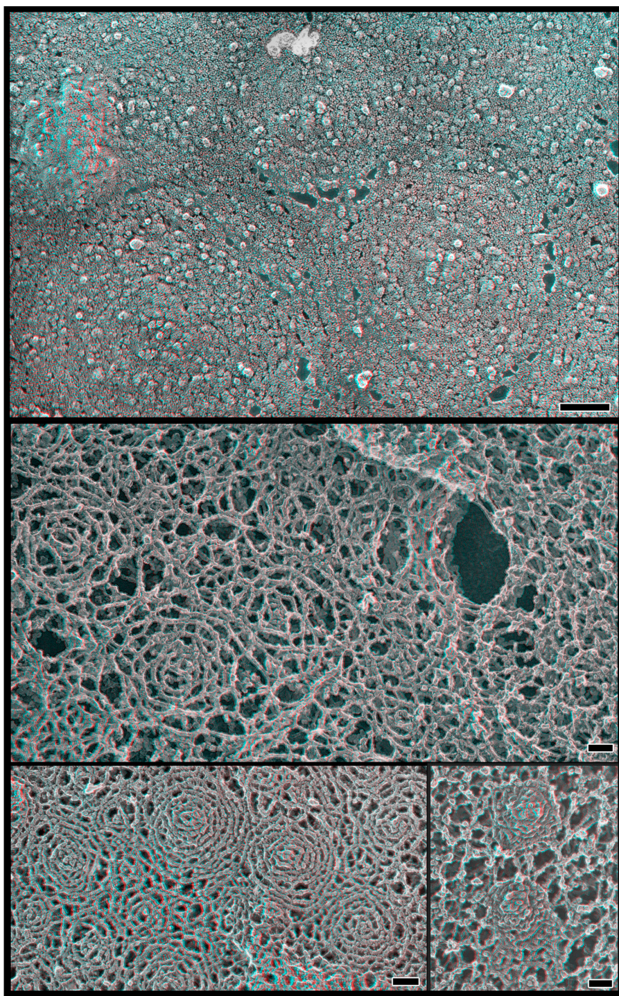
Figure 3. hSnf7 filaments on the top surface of the cell. (top) Patterns created by hSnf7-1 filaments on the outer surface of whole cells. Shown is the top surface of a COS-7 cell transfected with FLAG hSnf7-1, fixed, and replicated without disruption. Note the subtle circular patterning of particles within the membrane. (middle) Views of hSnf7-1 filaments in the subplasmalemmal "membrane skeleton" revealed by extracting fixed whole cells with detergent. The cell on the left expresses FLAG hSnf7-1, whereas the one on the right does not. (bottom left) Fixed and extracted cell expressing higher levels of FLAG hSnf7-1. (bottom right) Fixed and extracted cell expressing hSnf7-1-mGFP. Bars, 100 nm.
