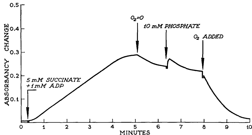
FIGURE 1 Demonstration of respiration-dependent changes in light scattering by water-washed rat liver mitochondria. Water-washed mitochondria were prepared and tested in air-saturated tris-MgCl 2 medium as described in the section on Methods. A time recording of the absorbancy changes under the conditions described in the text was made in a Cary model 14 recording spectrophotometer. A suspension of water-washed mitochondria in reaction mixture (approximately 2 mg protein per ml) was added to the reference and experimental cuvettes; this gave an initial absorbancy (or optical density) difference between the two samples which was almost negligible. Explanation of the additions made (to the experimental cuvette only) are given in the text.
