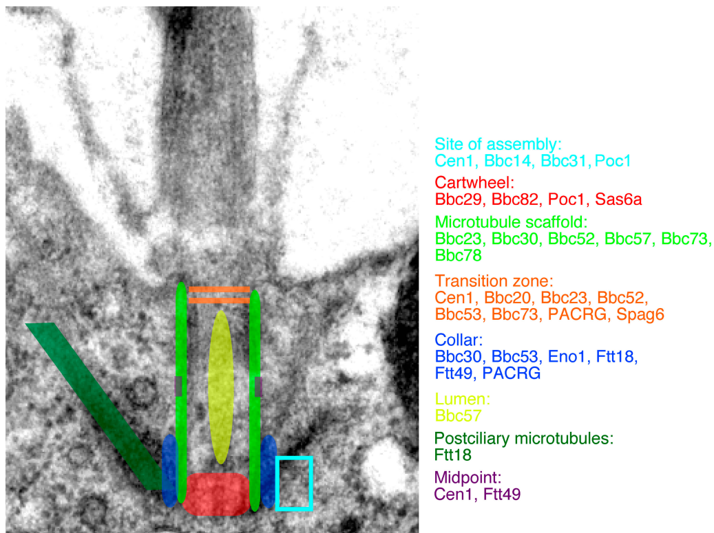
Figure 4. New T. thermophila basal body components were shown to localize to discrete structural domains. Protein localizations were assigned to specific domains if at least 20% of all gold particles in the immunoelectron microscopy compilation images are associated with the region. New protein components are listed in Fig. 2 B and in Figs. S1–3 (available at http://www.jcb.org/cgi/content/full/jcb.200703109/DC1 ). Color reference and domain are listed for each new basal body component described.
