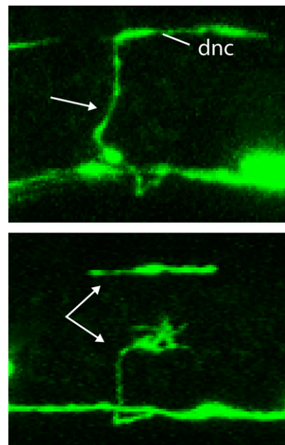
An axon (arrow) snaps (top to bottom) in a worm lacking \beta -spectrin.
