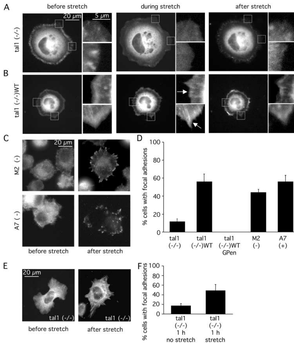
Figure 7. Talin1 is critical for the early integrin- and stretch-dependent formation of adhesion sites. (A) Representative stretching (10%) of talin1 (-/-) cells transiently transfected with paxillin-GFP. After 10 min of spreading, cells were stretched, held for 2 min, and subsequently relaxed by allowing the stretched silicone membrane to return to its original size. Before stretch (left), 2 min after stretch (middle), and after relaxation of stretch (right). Boxed areas are shown enlarged (right panels). (B) Representative stretching of talin1 (-/-) cells transiently transfected with the full-length talin1 and paxillin-GFP. As for talin1 (-/-) cells, no adhesion sites were visible in talin1 (-/-) WT cells before stretch (left). However, after 2-min stretch, adhesion sites were formed at the cell periphery visualized by paxillin-GFP fluorescence (arrows). Boxed areas are shown enlarged (right panels). (C) M2 (filaminA null) or A7 cells (stably expressing filaminA) were allowed to spread for 10 min and stretched for 2 min before fixation with 3.7% formaldehyde/PBS. M2 and A7 cells were subjected to immunostaining using antipaxillin antibody. (D) Summary of stretch-dependent formation of adhesion sites experiments during cell spreading. (E) Talin1 (-/-) cells transiently transfected with paxillin-GFP were allowed to spread for 1 h on pronectin-coated silicone membranes, and were stretched or not for 2 min before fixation. Representative localization of paxillin-GFP in talin1 (-/-) cells before stretch (left) and after stretch (right). (F) Summary of stretch-dependent formation of adhesion sites experiments after 1 h of cell spreading. (D and F) Results shown are the mean \pm SD of at least three independent experiments.
