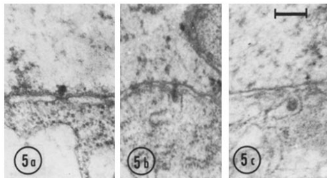
FIGURE 5 The occurrence of single 300–500- \text{\AA} RNP particles at the inside (a), within (b), and at the outside (c) of the nuclear membrane. Scale bar: 200 nm. \times 42,000.
