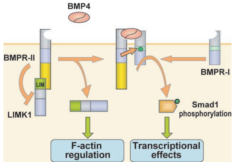
Figure 6. Schematic representation of two signaling outputs from the BMPR system. In the canonical Smad signaling process, BMP4 binds to and brings together BMPR-I (-IA or -IB, also known as ALK3 and ALK6, respectively) and BMPR-II. BMPR-II phosphorylates the regulatory region (green box) of BMPR-I, activating the kinase domain (blue box), which phosphorylates Smad1, leading to its nuclear translocation for regulation of target genes. The present results show that the COOH-terminal tail domain (yellow box) of BMPR-II in the basal state binds to the LIM domain region of LIMK1 and inhibits LIMK1. BMP4 binding relieves this inhibitory interaction, enabling LIMK1 to phosphorylate cofilin, thereby regulating the actin cytoskeleton.
