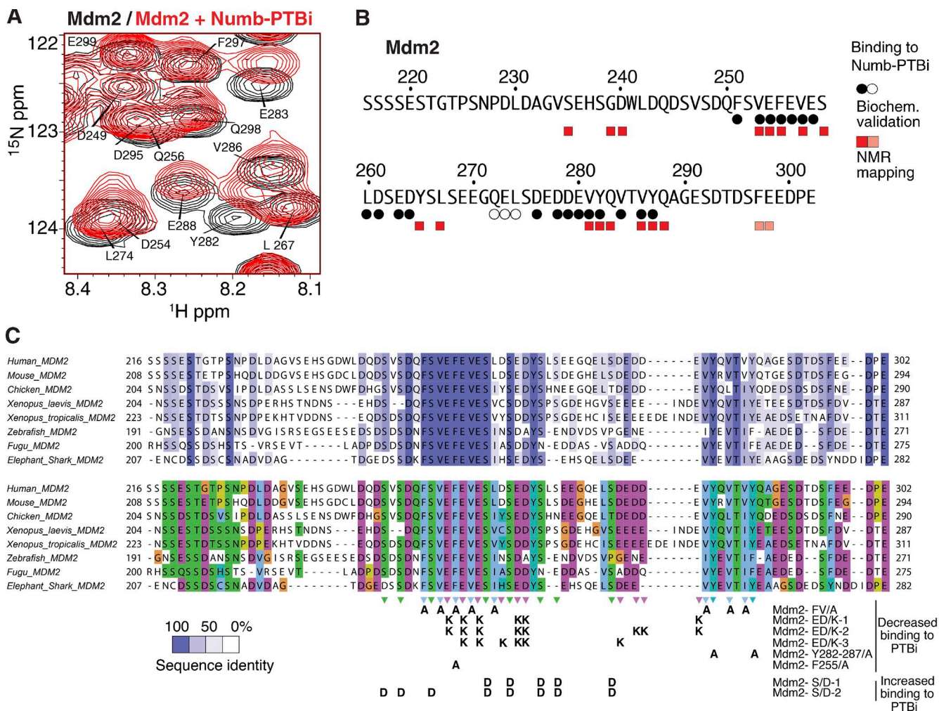
Figure 5. Characterization of the PTBi–Mdm2 interface on the Mdm2 side. (A) Region of [^1\text{H}][^{15}\text{N}] HSQC NMR spectra of [^{15}\text{N}] -labeled Mdm2 ^{216-302} free (black) or in the presence of 1.1 equivalents of PTBi (red). (B) Summary of the NMR spectral changes upon binding of PTBi to Mdm2 ^{216-302} . Residues which have a corresponding peak shift in the presence of Numb-PTBi are denoted with boxes with pink indicating 0.1–0.2 ppm and red indicating >0.2 ppm (see also Fig. S3 G). Results of the biochemical validation of Mdm2 residues at the interface with Numb-PTBi are shown in circles with the same color code as in Fig. 4 D (see also C and Fig. 6, A–F). (C) Summary of effects on binding to PTBi for all Mdm2 mutants tested. The mutants are shown aligned to a phylogenetic comparison among eight orthologues to evidence residue conservation and chemical nature of the residues. Top: Mdm2 residues are colored according to their conservation, which was calculated based on the alignment of eight orthologues from Homo sapiens , Mus musculus , Gallus gallus , Xenopus laevis , Xenopus tropicalis , Danio rerio (Zebrafish), Takifugu rubripes (Fugu), and Callorhynchus milii (Elephant shark). (Middle: same alignment as above, with colors reflecting the chemical nature of the side chains. Hydrophobic side chains are in blue, negatively charged are in purple, and Ser/Thr/Gln are in green. (Bottom: summary of the Mdm2 mutants used in binding assays of Fig. 6 (A–E) to characterize the Mdm2–Numb-PTBi interface.
