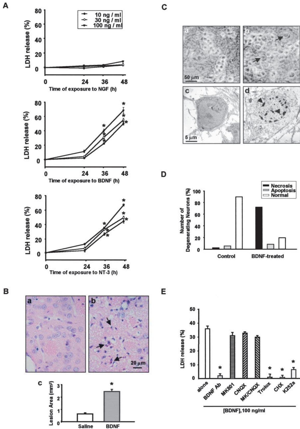
Figure 1. Prolonged exposure to NTs produces neuronal cell necrosis in cortical cell cultures. (A) Mixed cortical cell cultures (DIV 12–15) were continuously exposed to 10, 30, and 100 ng/ml of NGF, BDNF, or NT-3 for the indicated points of time. Neuronal cell death was assessed by measurement of LDH efflux to the bathing medium, mean \pm SEM ( n = 16 culture wells per condition). *Significant difference from the relevant control (sham washed control) at P < 0.05 using analysis of variance and Student-Neuman-Keuls test. (B) Brain sections were stained with hematoxylin-eosin at 2 d after intrastriatal injections of 5 \mu l of saline or 5 \mu g BDNF. Bright field photomicrographs showing a representative striatal area 1 mm lateral to the injection site of saline (a) or BDNF (b). Note the pyknotic neurons (arrows) in BDNF-treated
