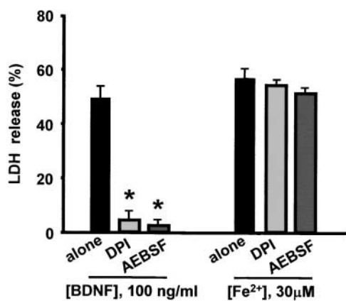
Figure 6. Activation of NADPH oxidase mediates BDNF-induced neuronal death. Cortical cell cultures (DIV 12–15) were exposed to 100 ng/ml BDNF or 30 μM Fe 2+ , alone or in the presence of 3 nM DPI or 10 μM AEBSF. Neuronal death was analyzed 36 h later by measurement of LDH efflux into the bathing medium, mean ± SEM ( n = 16 culture wells per condition). *Significant difference from the relevant control (BDNF or Fe 2+ alone) at P < 0.05 by Student-Neuman-Keuls test.
