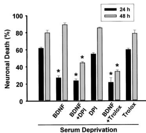
Figure 7. DPI or trolox enhances the neuroprotective effect of BDNF against serum deprivation. Neuron-rich cortical cell cultures (DIV 7) were deprived of serum, alone (serum deprivation) or in the presence of 100 ng/ml BDNF, 100 ng/ml BDNF plus 3 nM DPI, 3 nM DPI, 100 ng/ml BDNF plus 100 μM trolox, or 100 μM trolox. Neuronal death was assessed 24 and 48 h later by counting viable neurons, mean ± SEM ( n = 16 fields randomly chosen from four culture wells per condition). *Significant difference from the relevant control (serum deprivation alone) at P < 0.05 using analysis of variance and Student-Neuman-Keuls test.
