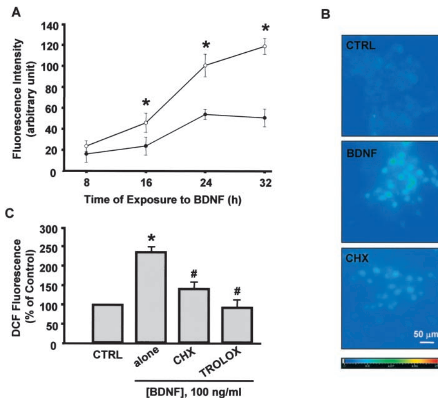
Figure 2. BDNF produces ROS in cortical neurons: involvement of protein synthesis. (A) Cortical cell cultures (DIV 12–15) were exposed to a sham wash (●) or 100 ng/ml BDNF (○). Levels of ROS in neurons were analyzed at indicated times by measuring fluorescence intensity of oxidized DCFH-DA (DCF), mean \pm SEM ( n = 30 – 35 neurons randomly chosen from four culture wells per condition). *Significant difference from the relevant control (sham wash) at P < 0.05 using analysis of variance and Student-Neuman-Keuls test. (B and C) Fluorescence photomicrographs (B) and quantitation (C) of DCF in cortical neurons after 32 h exposure of cortical cell cultures (DIV 12–15) to a sham wash (CTRL) or 100 ng/ml BDNF, alone (BDNF) or in the presence of 1 \mu M cycloheximide (CHX) or 100 \mu M trolox (TROLOX). *Significant difference from the control (CTRL); #significant difference from the BDNF control (BDNF alone) at P < 0.05 using analysis of variance and Student-Neuman-Keuls test.
