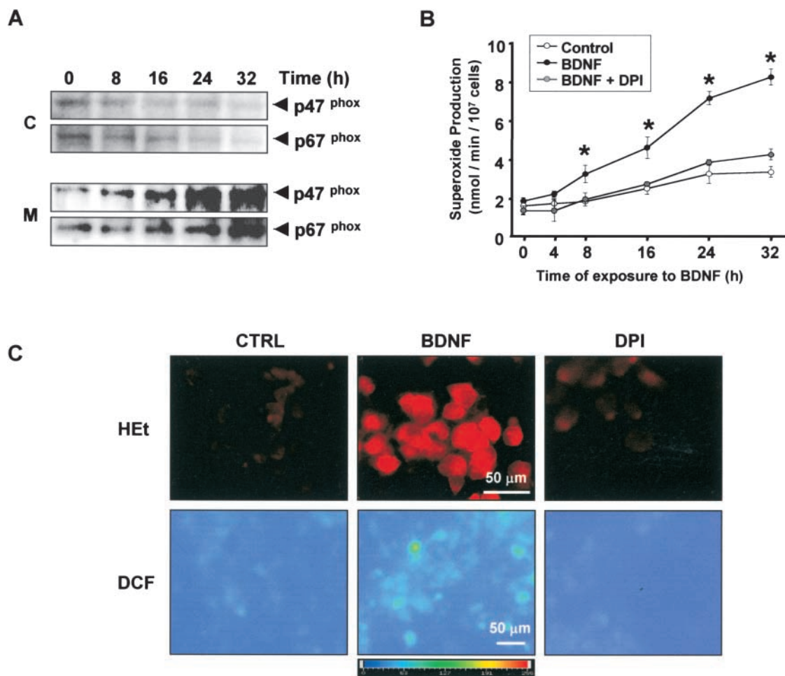
Figure 5. Translocation and activation of NADPH oxidase by BDNF. (A) Western blot analysis of the cytosolic fraction (C) and the membrane fraction (M) using anti-p47-phox and anti-p67-phox antibodies that were obtained from cortical cell cultures (DIV 12) after exposure to 100 ng/ml BDNF for the indicated times. (B) Superoxide production was analyzed by measuring reduction of cytochrome c in cortical cultures exposed to a sham wash (○) or 100 ng/ml BDNF with (gray colored circles) or without 3 nM DPI (●) for indicated times, mean \pm SEM ( n = 12 culture wells per condition). *Significant difference from the sham control at P < 0.05 using analysis of variance and Student-Neuman-Keuls test. (C) Fluorescence photomicrograph of the oxidized hydroethidine (HEt, top) and DCF (bottom) in cortical neurons after exposure to a sham operation (CTRL), 100 ng/ml BDNF (BDNF), or 100 ng/ml BDNF plus 3 nM DPI (DPI) for 32 h.
