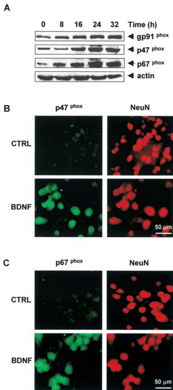
Figure 4. BDNF increases expression of NADPH oxidase subunits in cortical neurons. (A) Western blot analysis of NADPH oxidase subunits (gp91-phox, p47-phox, and p67-phox) and actin in cortical cell cultures after exposure to 100 ng/ml BDNF for indicated times. Similar results were obtained from three separate experiments. (B) Fluorescence photomicrograph of cortical cell cultures immunolabeled with NeuN (right; anti-mouse immunoglobulin G conjugated with Texas red) and anti-p47-phox (left; anti-goat immunoglobulin G conjugated with FITC) after exposure to a sham wash (top) and 100 ng/ml BDNF (bottom) for 32 h. (C) Same as B except that cultures were immunolabeled with anti-p67-phox antibody (anti-goat immunoglobulin G conjugated with FITC) instead of anti-p47-phox. Note that levels of p47-phox and p67-phox were increased selectively in neurons after exposure of mixed cortical cell cultures to BDNF.
