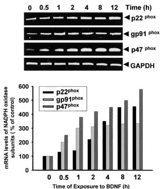
Figure 3. BDNF increases mRNA levels of NADPH oxidase subunits in cortical cultures. RT-PCR analysis of NADPH oxidase subunits (p22-phox, gp91-phox, and p47-phox) and GAPDH mRNA expression in cortical cell cultures (DIV 12) exposed to 100 ng/ml BDNF for indicated times. The mRNA level of each NADPH oxidase subunit was normalized to the relevant control value ( t = 0 ). Similar results were observed from three separate experiments.
