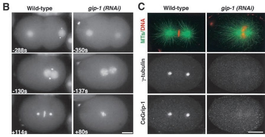
Figure 4. Depletion of CeGrip-1 blocks recruitment of centrosomal \gamma -tubulin. (A) CeGrip-1 contains the two grip motifs found in proteins that form complexes with \gamma -tubulin (Gunawardane et al., 2000). By performing further BLAST searches using the grip motifs as a query sequence, we recently identified a second predicted C. elegans protein, CeGrip-2 (C45G3.3), that contains the grip motifs. Here, grip motifs 1 and 2 from CeGrip-1 and CeGrip-2 are aligned with the grip motifs from other proteins homologous to Dgrip91/Spc98p. Amino acids conserved in 80–100% of the sequences are highlighted in yellow. The conserved amino acids that define grip motifs 1 and 2 (Gunawardane et al., 2000) are shown beneath the alignments in red and green, respectively. (B) Panels summarizing a time-lapse sequence of a wild-type (left) and a gip-1(RNAi) embryo (right) expressing both GFP–histone and GFP– \gamma -tubulin. In gip-1(RNAi) embryos, the \gamma -tubulin signal was greatly reduced or, as in this case, absent (see Videos 1 and 2 located at http://www.jcb.org/cgi/content/full/jcb.200202047/DC1 ). (C) Mitotic wild-type and gip-1(RNAi) embryos stained for MTs and DNA (green and red, top), \gamma -tubulin (middle), and CeGrip (bottom) are shown. CeGrip-1 and \gamma -tubulin colocalize at centrosomes. Depletion of CeGrip-1 prevents \gamma -tubulin recruitment to centrosomes and results in an MT phenotype essentially identical to that observed in tbg-1(RNAi) embryos. Depletion of CeGrip-2 also results in an MT phenotype essentially identical to that in tbg-1(RNAi) embryos (unpublished data). Bars, 10 \mu m.
