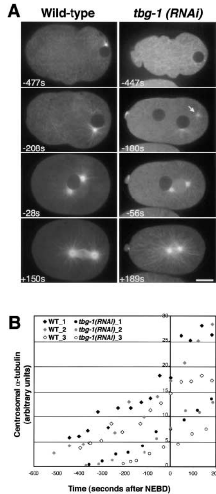
Figure 5. During mitosis in tbg-1(RNAi) embryos, centrosomal \alpha -tubulin fluorescence reaches \sim 40\% of wild-type levels. (A) Panels summarizing movies of wild-type (left) and tbg-1(RNAi) embryos (right), expressing GFP- \alpha -tubulin. Times are with respect to NEBD. See also Videos 3 and 4 located at http://www.jcb.org/cgi/content/full/jcb.200202047/DC1 . In wild type, asters are visible at an early stage ( -477 s). The asters grow in size (all panels) and become the poles of the mitotic spindle ( +150 s). ( -447 s) In tbg-1(RNAi) embryos there are no detectable asters at early time points. ( -180 s) Coincident with the onset of mitotic prophase in wild-type (judged by comparison of GFP- \alpha -tubulin and GFP-histone sequences), centrosomal asters form in the tbg-1(RNAi) embryos. At this time, centrosomes (arrow) are often observed to "fly in" to meet the paternal pronucleus. ( +189 s) After NEBD, robust mitotic asters form but no spindle assembles. Bar, 10 \mu\text{m} . (B) Kinetic traces of centrosomal \alpha -tubulin fluorescence. Centrosomal fluorescence was quantitated in five wild-type and four tbg-1(RNAi) embryos. Three traces are shown for each.
