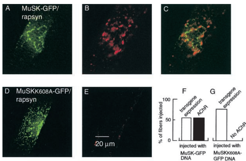
Figure 3. Induction of ectopic AChR clusters requires MuSK kinase activity. Rat muscle fibers were injected with expression vectors encoding MuSK-GFP or MuSK K608A -GFP and rapsyn. After 21 d, the muscles were excised. Maximum
