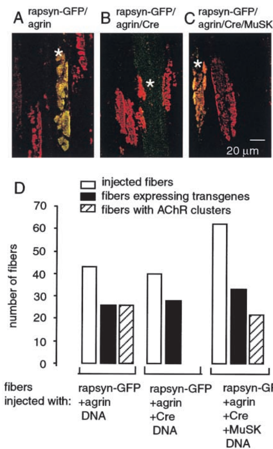
Figure 5. Rapsyn-GFP identifies ectopically induced AChR clusters. Single muscle fibers of MuSK loxP/- mice were injected with DNA, as indicated by asterisks, and expression of transgenic products was analyzed 21 d after injection. The excised muscles were incubated with r-bgt to identify AChR clusters. Overlays of green and red fluorescence images of a confocal image series are shown as maximum projections. (A) Expression of agrin and rapsyn-GFP as indicated. Agrin induces ectopic AChR clusters. AChR in the injected muscle fiber form complexes with rapsyn-GFP and AChR clusters appear yellow in the overlay. The r-bgt labeled AChR clusters on noninjected fibers are red. (2 MuSK loxP/- mice were used for injection; a total of 43 fibers were injected and 26 fibers expressed agrin and rapsyn-GFP. In all injected transgene-expressing fibers AChRs were colocalized with rapsyn-GFP and appeared yellow). (B) Expression of agrin, Cre, and rapsyn-GFP as indicated. Transgenic Cre inactivates endogenous MuSK. The absence of AChR/rapsyn-GFP clusters demonstrates that the formation of AChR clusters was prevented in injected muscle fibers. Agrin-induced AChR clusters are found only on neighboring noninjected fibers. 2 MuSK loxP/- mice were used for DNA injection; a total of 40 fibers were injected; 28 fibers expressed agrin and rapsyn-GFP; no AChR clusters were detected on the injected fibers. (C) Expression of agrin, Cre, rapsyn-GFP, and MuSK as indicated. AChR induced in the injected fiber form complexes with rapsyn-GFP and AChR clusters appear yellow in the overlay. The Cre-mediated inactivation of the MuSK gene was rescued by expression of transgenic MuSK (3 MuSK loxP/- mice were used for DNA injection; a total of 62 fibers were injected and 33 fibers expressed agrin and rapsyn-GFP. Endogenous MuSK inactivation was rescued in 22 fibers, which contained AChR/rapsyn-GFP complexes.) (D) Graphic summary of experiments described in A–C shows that Cre-mediated inactivation of endogenous MuSK prevents the formation of AChR clusters. The conditional MuSK gene knock out is rescued with high efficiency by transgenic MuSK: AChR clusters are found in 73% of transgene-expressing fibers.
