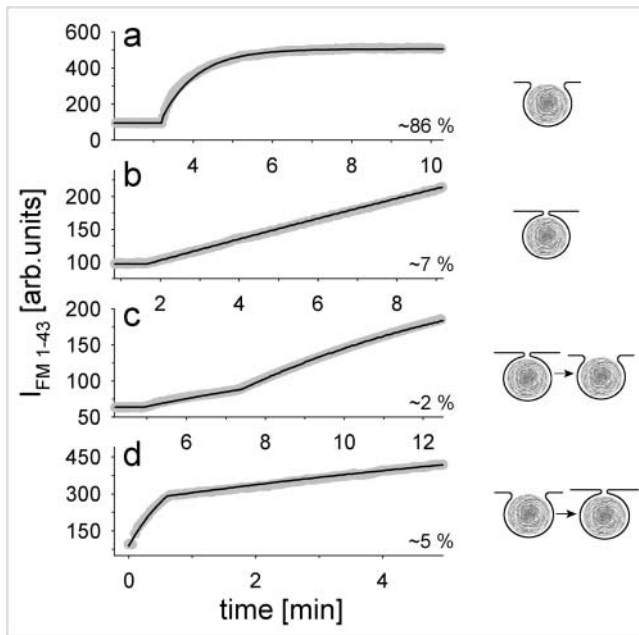
Figure 3. Initial states of fusion pores in caged \text{Ca}^{2+} -stimulated fusions. Fast exponential (a), slow gradual (b), and biphasic (c and d) I_{\text{FM}1-43} developments were observed at the indicated frequencies ( n = 80 ; flash photolysis was done at time 0). Data (gray circles) were fit by Eq. A4 (solid lines), allowing to calculate fusion pore diameters for each experiment (see text).
