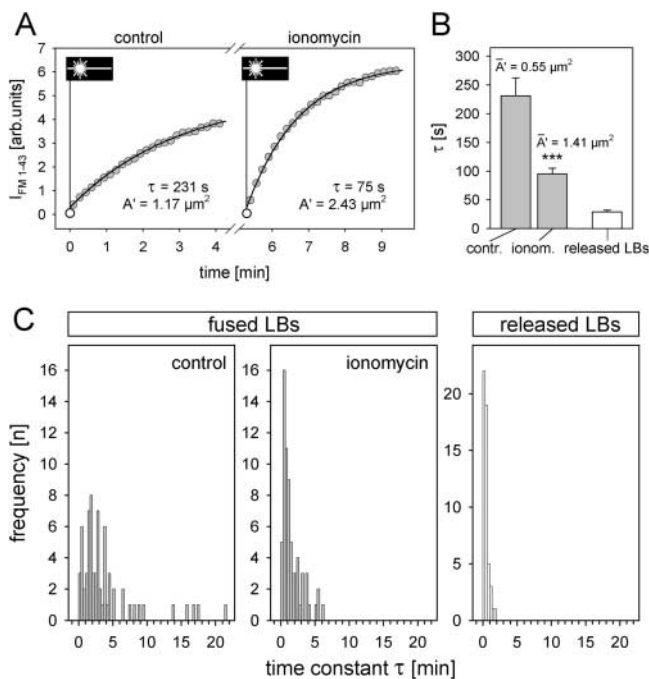
Figure 6. Ca^{2+} effect on fusion pores. (A) Repeated FRAP of a single LB before (control) and after treatment with ionomycin. Time of photobleaching is indicated by the laser symbol. Data were fit by Eq. A4, revealing a decrease in \tau and, correspondingly, an increase in the pore area. (B) Averaged time constants derived from measurements exemplified in A ( n = 68 ; P < 0.001 ), and from released LBs. According to our model, and using an experimentally determined mean LB \varnothing of 1.68\ \mu m , these values yield an increase in mean pore area ( A' ) after treatment with ionomycin as indicated. (C) Frequency distribution of time constants in fused (before and after ionomycin treatment) and released LBs. These data were used for the calculations shown in B.
