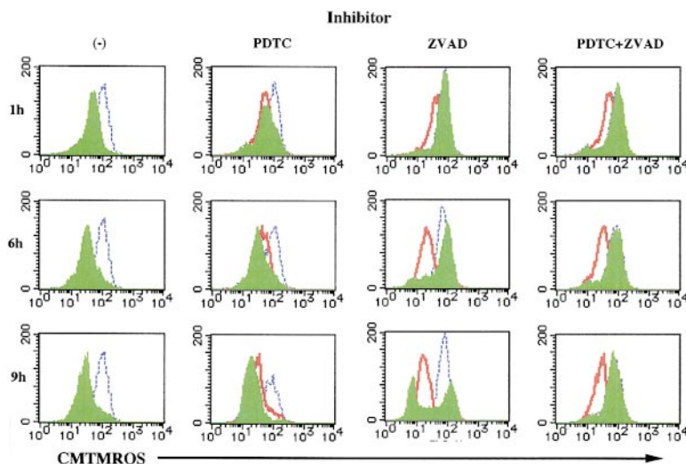
Figure 5. Inhibitory effects of PDTC and z-VAD-fmk on Fas-induced reduction of the \Delta\Psi\text{m} . JmF cells ( 10^6 cells/ml) were incubated at 37°C with 1 \mu\text{g/ml} Jo2 antibody alone (first column) or in the presence of 80 \mu\text{M} PDTC (second column), 0.5 mM z-VAD-fmk (third column), or 80 \mu\text{M} PDTC and 0.5 mM z-VAD-fmk (fourth column). After incubation for the indicated time periods (shown to the left of each row), \Delta\Psi\text{m} was measured, as described in Materials and Methods. The FACS ® profiles are shown in the green areas. The FACS ® profiles of cells without anti-Fas antibody treatment are indicated by open areas with dotted lines in all panels, whereas those obtained without inhibitors are indicated by open areas with red lines in the panels of the second, third, and fourth columns.
