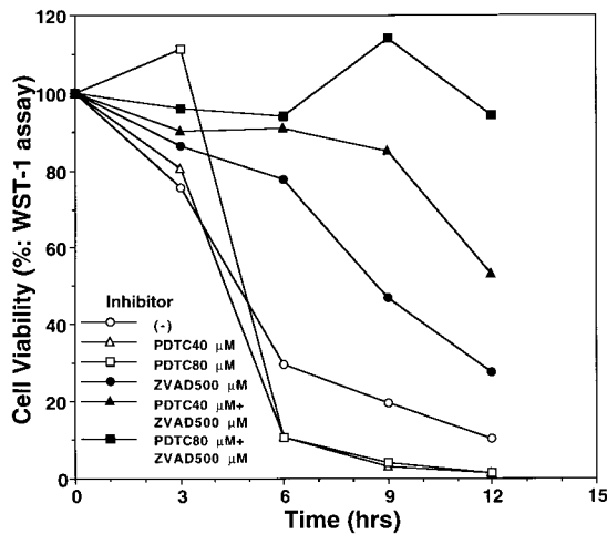
Figure 4. Inhibitory effects of a caspase inhibitor and PDTC on the Fas-induced cell death. JmF cells were incubated with 1 \mu\text{g/ml} Jo2 antibody alone ( \circ ) or in the presence of 40 \mu\text{M} PDTC ( \Delta ), 80 \mu\text{M} PDTC ( \square ), 0.5 mM z-VAD-fmk ( \bullet ), 40 \mu\text{M} PDTC and 0.5 mM z-VAD-fmk ( \blacktriangle ), and 80 \mu\text{M} PDTC and 0.5 mM z-VAD-fmk ( \blacksquare ). After incubation at 37°C for the indicated time periods, cell viability was determined by the WST-1 assay, as described in Materials and Methods. The results are expressed as the percent of the value obtained without the Jo-2 antibody. The experiments were performed in triplicate, and the average values were plotted.
