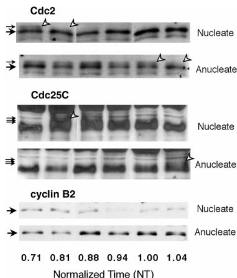
Figure 2. MPF activation is delayed in anucleate egg fragments. Small groups of nucleate and anucleate fragments were frozen at different times, processed for Western blotting, and probed with antibodies to detect Cdc2, Cdc25C, and cyclin B2. Approximately 0.2 egg volume equivalents were loaded in each lane. For each blot shown (as well as for those in the figures following), different molecular weight regions of the same blot were probed with the appropriate antibody. Cdc2 was detected with anti-PSTAIR antibody. The small black arrows indicate the phosphorylated (upper, inactive) isoform and the large black arrows the lower isoforms of Cdc2. The lower bands include both the inactive non-T14/Y15–phosphorylated isoform and the active T14/Y15–dephosphorylated isoform. The white arrowheads indicate the maximal detected phosphorylation and the beginning of dephosphorylation of Cdc2 (MPF activation). For Cdc25C, the small arrows mark the phosphorylated isoforms, which appear upon Cdc25C activation (white arrowheads). Activation of both Cdc2 and Cdc25C was delayed by \sim 0.25 time units in anucleate fragments. Cyclin B2 accumulated similarly in both fragments until \sim 0.8 NT, after which time it was degraded in nucleate but not in anucleate fragments. Reaccumulation of cyclin B2 in the second cycle is first detectable in nucleate fragments at the time of cleavage.
