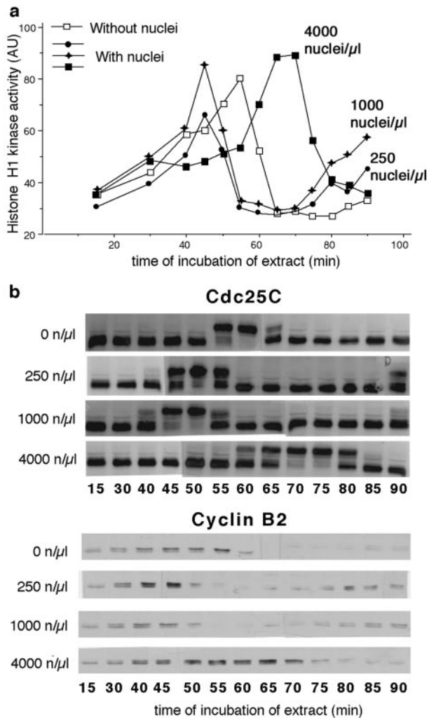
Figure 3. Nuclei stimulate MPF activation in vitro. (a) Histone H1 kinase activity during the first cell cycle of a Xenopus extract made 20 min after egg activation. Increasing volumes (0–8 \mu l) of nucleus suspension were added to 200 \mu l aliquots of the extract to give 0, 250, 1,000, and 4,000 nuclei/ \mu l of extract, then divided into 10 \mu l aliquots, incubated at 21°C, and samples were taken at 5-min intervals over a 90-min period. 250 and 1,000 nuclei/ \mu l advanced the peak of MPF activation by 10 min compared with extracts without nuclei. The delayed MPF activation in the presence of 4,000 nuclei/ \mu l is explained by the activation of the DNA replication checkpoint (Dasso and Newport, 1990). (b) Western blot performed with the same samples using anti-Cdc25C and anti-cyclin B2 antibodies. Maximum phosphorylation of Cdc25C and peak cyclin B2 coincided with peak H1 kinase activity.
