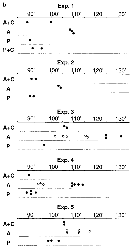
Figure 8. Centrosome injection into anucleate eggs advances SCWs. (a) Experimental design. Definitive assignment of egg categories was made at the end of each experiment based on cleavage pattern (see text). A, anucleate eggs; A+C, anucleate egg with centrosomes; P, prick-activated eggs; P+C, prick-activated eggs with centrosomes. (b) Comparison of timing of the first SCW in different egg categories in five separate experiments. Filled circles indicate the time (minutes after activation) that the first SCW crossed the vegetal hemisphere. Open circles represent the time of exaggerated germ plasm aggregation starting at the end of the cortical rotation seen in anucleate eggs in three experiments, which preceded characteristic SCWs in two of these experiments. Enucleation success for experiments (Exp.) 1, 2, 3, and 4 was 60%, and for experiment 5 was 75% (assessed from groups of 10–20 eggs cultured in parallel).
