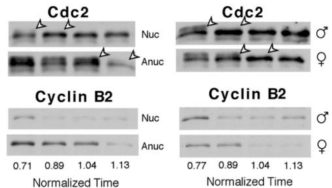
Figure 5. MPF activation depends on nuclei and centrosomes. Cdc2 and cyclin B2 proteins followed by Western blotting (see Fig. 2) in nucleate (Nuc) and anucleate (Anuc) fragments compared with fragments containing a single male or female pronucleus. The centrosome associated with the male pronucleus organizes a microtubule aster. Cdc2 dephosphorylation was first detectable in fragments containing both nuclei and asters, then in fragments containing the female pronucleus, and finally in anucleate fragments. Low cyclin B2 levels in the last lane of anucleate samples (left blot) partially reflects reduced loading levels (compare with Cdc2 band intensities).
