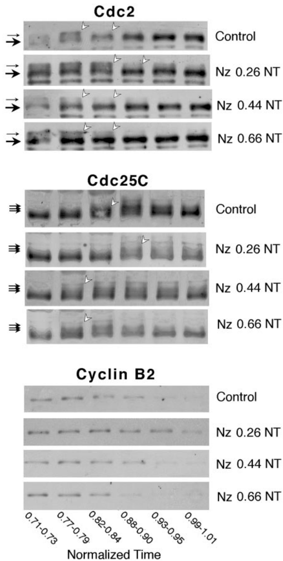
Figure 4. Early nocodazole treatment delays MPF activation. Western blots (details and annotations as in the legend to Fig. 2) showing the behavior of Cdc2, Cdc25C, and cyclin B2 during first mitosis after treatment at different times with 10 mM nocodazole. Treatments were started at 0.26, 0.44, and 0.66 NT as indicated. The times below each lane show the period of collection and freezing of control and treated eggs. Eggs treated at 0.26 NT showed a delay in Cdc2 and Cdc25C activation of \sim 0.1 time units, whereas treatments beginning at 0.44 and 0.66 NT did not. Degradation of cyclin B2 was delayed in the early nocodazole-treated eggs and appeared to degrade more slowly.
