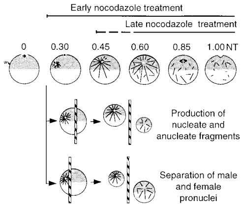
Figure 1. Dissection of the role of nuclei and microtubules in MPF activation in Xenopus eggs. Diagram showing the different experimental protocols used, in relation to the changing microtubule organization throughout the first cell cycle (Houliston and Elinson, 1992). The centriole, brought by the sperm, recruits cytoplasmic components to form an active centrosome that nucleates a giant microtubule aster, which is first manifest by pigment accumulation around the sperm entry point in the animal cortex between 0.2 and 0.3 NT. The sperm aster mediates the migration of both male and female pronuclei to the center of the animal hemisphere where they are found closely apposed at \sim 0.5 NT. At this time, general microtubule polymerization occurs throughout the egg. At \sim 0.8 NT, the mitotic spindle forms in the animal hemisphere whereas cytoplasmic microtubules depolymerize. At 1.0 NT, the cleavage furrow is initiated at the animal pole. Early nocodazole treatments started between 0.2 and 0.3 NT to prevent sperm aster growth, and late treatments around 0.45 or 0.65 NT to eliminate microtubules at the time of mitosis. Nucleate and anucleate fragments were separated by placing glass rods to one side of the animal pole, thus generating a larger fragment containing the sperm aster and nuclei, and the smaller anucleate fragment. Alternatively, the rod was placed between the animal pole and the sperm entry point to produce one small fragment with the male pronucleus and attached centrosome, and a large fragment containing just the female pronucleus.
