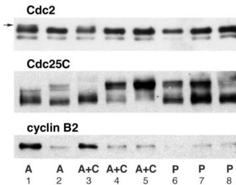
Figure 9. Centrosome injection into anucleate eggs stimulates MPF activation. Cdc2/Cdc25C/Cyclin B2 blots (details and annotations as in the legend to Fig. 2) of single eggs harvested simultaneously 88 min after activation from an equivalent experiment to that described in the legend to Fig. 8. At this time, the “anucleate” (A) egg in track 1 contained preactive MPF as shown by the presence of inactive Cdc2 isoforms (arrow) and cyclin B2. The “anucleate” centriole-injected (A+C) egg in lane 3 was in an equivalent premitotic state; however, the other two were strongly mitotic, with no detectable inactive, phosphorylated Cdc2, and highly phosphorylated Cdc25C. In contrast, the three prick-activated (P) eggs (lanes 6–8) have all passed through mitosis, as indicated by the partial dephosphorylation of Cdc25C and absence of cyclin B2. The migration of the three proteins in the A egg in lane 2 resembles the activated eggs, suggesting that enucleation was probably unsuccessful.
