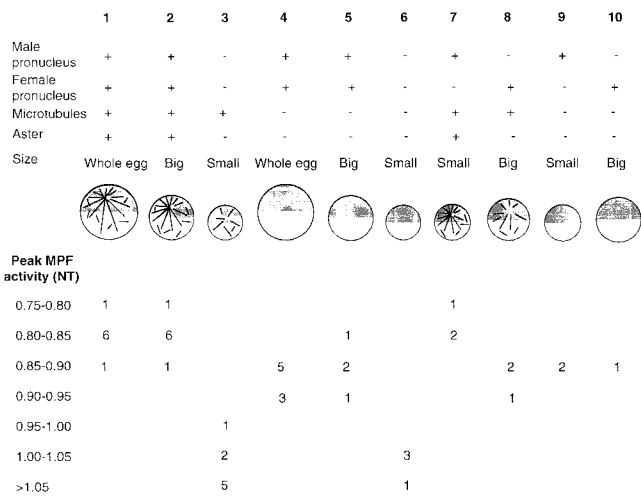
Figure 6. Additive effects of microtubules, nuclei, and centrosomes in vivo. Combined data from ligation and nocodazole experiments in which the timing of MPF activation was assessed from blots of groups of fragments frozen at successive times with antibodies recognizing Cdc2, cyclin B2, and Cdc25C. The number of cases in which MPF activation was detected during each time interval is indicated for each category.
