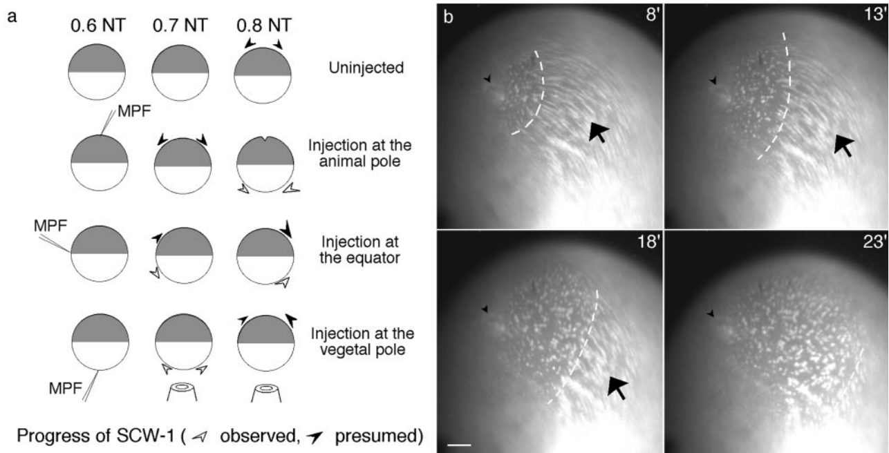
Figure 7. MPF injection provokes waves of cortical reorganization. (a) Diagram summarizing the effects of precocious injection of active MPF (human recombinant Cdc2-cyclin B) into different sites of fertilized eggs during interphase (0.6 NT). Animal pole injections ( n = 2 ) provoked premature SCWs and cleavage furrow formation. Injection in the equatorial region ( n = 2 ) and vegetal pole ( n = 8 ) produced waves propagating from the injection point that were similar in appearance, although not identical to the first SCW. (b) Superimposed sequences of 10 consecutive images from 1 recording showing the wave of cortical reorganization produced by vegetal injection of MPF. White stained dots are mitochondrial islands labeled with DiOC 6 (3). These translocate in a coordinate fashion indicating the direction of the cortical rotation relative to the cytoplasm (arrow). The cortical rotation was progressively stopped by the passage of a wave, similar to the first SCW, propagating from the point of injection (arrowhead). The time after injection in minutes is indicated. This ectopic wave is visible as a front of stationary germ plasm islands (dashed line). Bar, 100 \mu m.
