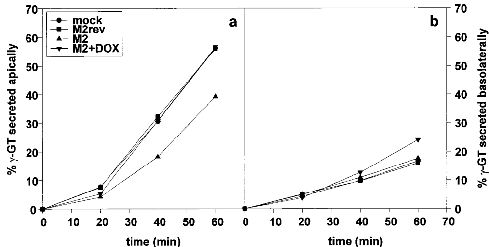
Figure 3. M2 slows apical but not basolateral delivery of a secreted form of \gamma -glutamyl-transpeptidase. MDCK cells stably expressing gD \gamma -GT were mock-infected or infected with AV-TA and either AV-M2rev or AV-M2. Indicated filters were treated with doxycycline (DOX) to block M2 expression. The following day, cells were radiolabeled, chased for 2 h at 19°C, then warmed to 37°C, and the release of \gamma -GT into the apical (a) and basolateral (b) medium was quantitated as described in Materials and Methods. Similar results were obtained in three experiments.
