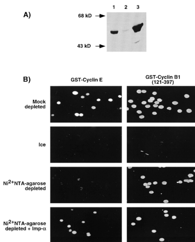
Figure 3. Nuclear import of GST-cyclin E, but not GST-cyclin B1 (121–397), requires importin- \alpha . (A) Ni 2+ NTA-agarose can be used to deplete importin- \alpha from egg cytosol. Anti-importin- \alpha Western blot for mock (Sephacrose CL-4B)-depleted (lane 1), Ni 2+ NTA-agarose-depleted (lane 2), and Ni 2+ NTA-agarose-depleted extract to which excess recombinant importin- \alpha (100 \mu g/ml) had been added back (lane 3). (B) Uptake assays into digitonin-permeabilized cells were performed for fluorescein maleimide-labeled GST-cyclin E and GST-cyclin B1 (121–397) with mock-depleted extract (passed over Sepharose CL-6B beads) at both room temperature and on ice, and at room temperature with Ni 2+ NTA-agarose-depleted extract. All assays contained the same final protein concentration of extract (4 mg/ml). Recombinant importin- \alpha , 50 \mu g/ml, was added back to a set of assays performed with Ni 2+ NTA-agarose-depleted extract to show that the effect of depletion on import was due primarily to the removal of importin- \alpha .
