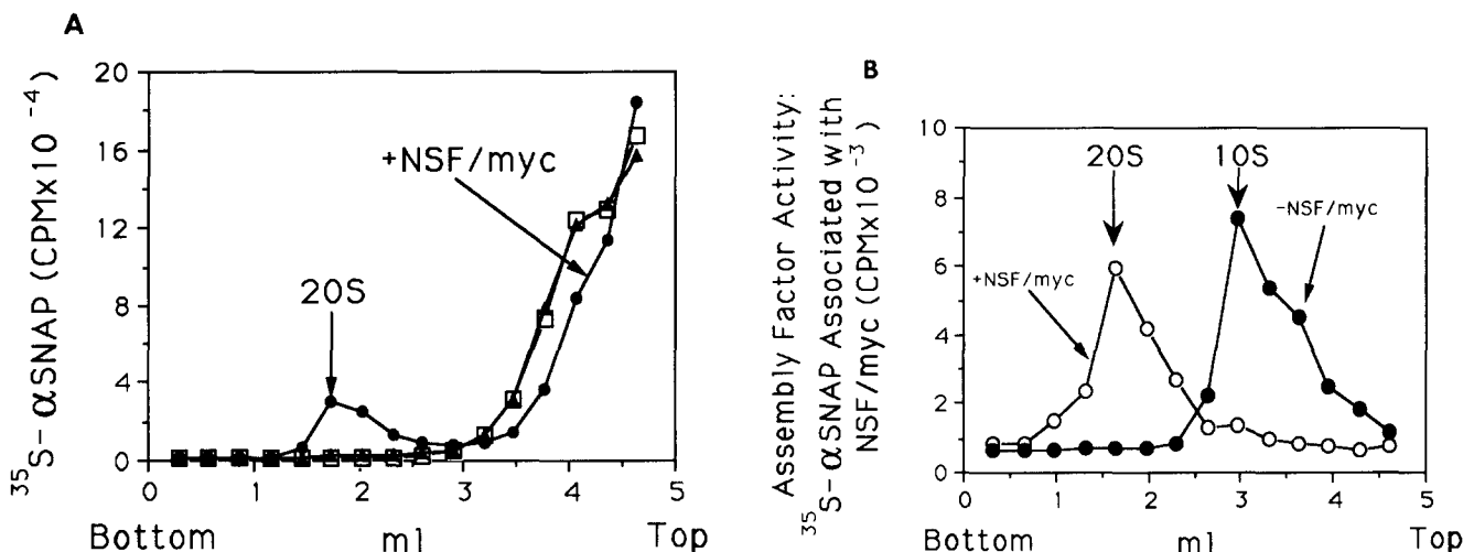
Figure 2. NSF/myc, \alpha -SNAP, and assembly factor form a 20S complex. (A) Detergent extracts of salt-washed RLG membranes were incubated with ^{35}\text{S} - \alpha -SNAP, NSF/myc (●), NEM-inactivated NSF/myc (▲) or no NSF/myc (□) and then sedimented through 10–35% glycerol (wt/vol) gradients. The position corresponding to a sedimentation coefficient of 20S is indicated. (B) Non-radioactive SNAP proteins (purified as described by Clary and Rothman, 1990), a detergent extract of salt-washed RLG membranes and NSF/myc (○) or buffer (●) were incubated to form a complex then subjected to sedimentation as in A. Gradient fractions were tested for assembly factor using a standard coimmunoprecipitation assay. Positions corresponding to sedimentation coefficients of 10S and 20S are indicated.
