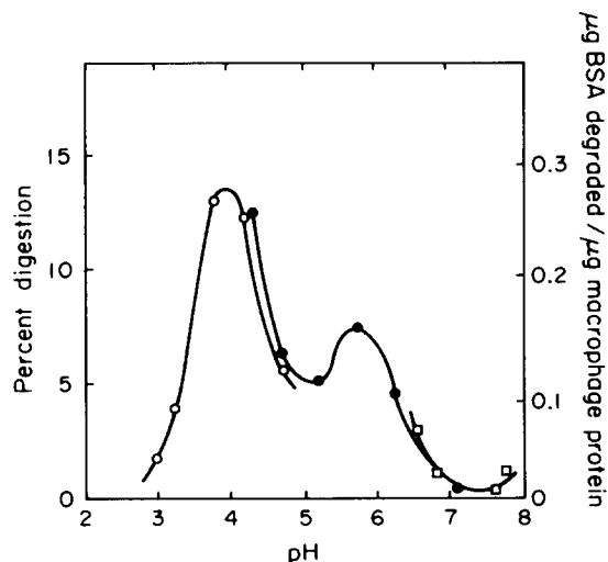
Figure 3. pH-dependence of the digestion of BSA by macrophage extracts. \circ , Na-lactate buffer; \bullet , Na-acetate buffer; \square , Na-phosphate buffer.
