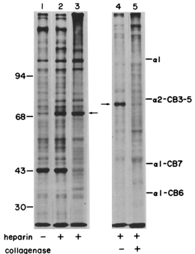
FIGURE 2 Induction of short-chain collagen by heparin. Multilayered SMC were treated with 100 \mu\text{g/ml} heparin in control culture medium (Waymouth's plus 10% fetal calf serum) for 72 h. Cultures were then metabolically labeled with [ ^3\text{H} ]proline in medium containing heparin but lacking serum for 24 h. Radiolabeled cell layer proteins were harvested into protease inhibitors and prepared for SDS PAGE and visualization by fluorography. Equal amounts of radioactivity were applied to lanes 1–3 and to lanes 4 and 5. Lane 1, control cell layers. Lane 2, cell layer proteins after treatment of cells with heparin. Note increased density of a band migrating with an apparent M_r = 70,000 (arrow), according to globular protein standards as shown to the left ( M_r \times 10^{-3} ). Lane 3, heparin-treated SMC cell layer proteins run under nonreducing conditions. All other lanes were run in the presence of dithiothreitol. Reducing agents do not affect the migration of the heparin-induced protein. Lanes 4 and 5 specific digestion of the heparin-inducible protein with bacterial collagenase. Radiolabeled cell layer proteins were harvested into protease inhibitors as described, incubated with bacterial collagenase for 90 min at 37°C, reprecipitated, and prepared, on a different gel than lanes 1–3, for SDS PAGE and fluorography. Cell layer proteins incubated with buffer alone (lane 4) or with collagenase (lane 5) are shown. Shown to the right are positions of migration of type I collagen standards. Indicated are relative mobilities of the \alpha 1 chain ( M_r 94,000), the CNBr cleavage products \alpha 2 -CB3–5 ( M_r 63,300), \alpha 1 -CB7 ( M_r 24,700), \alpha 1 -CB6 ( M_r 17,600), and the SMC collagen (arrow). The heparin-inducible collagen exhibits an apparent molecular weight, based on SDS PAGE analysis, of 60,000.
