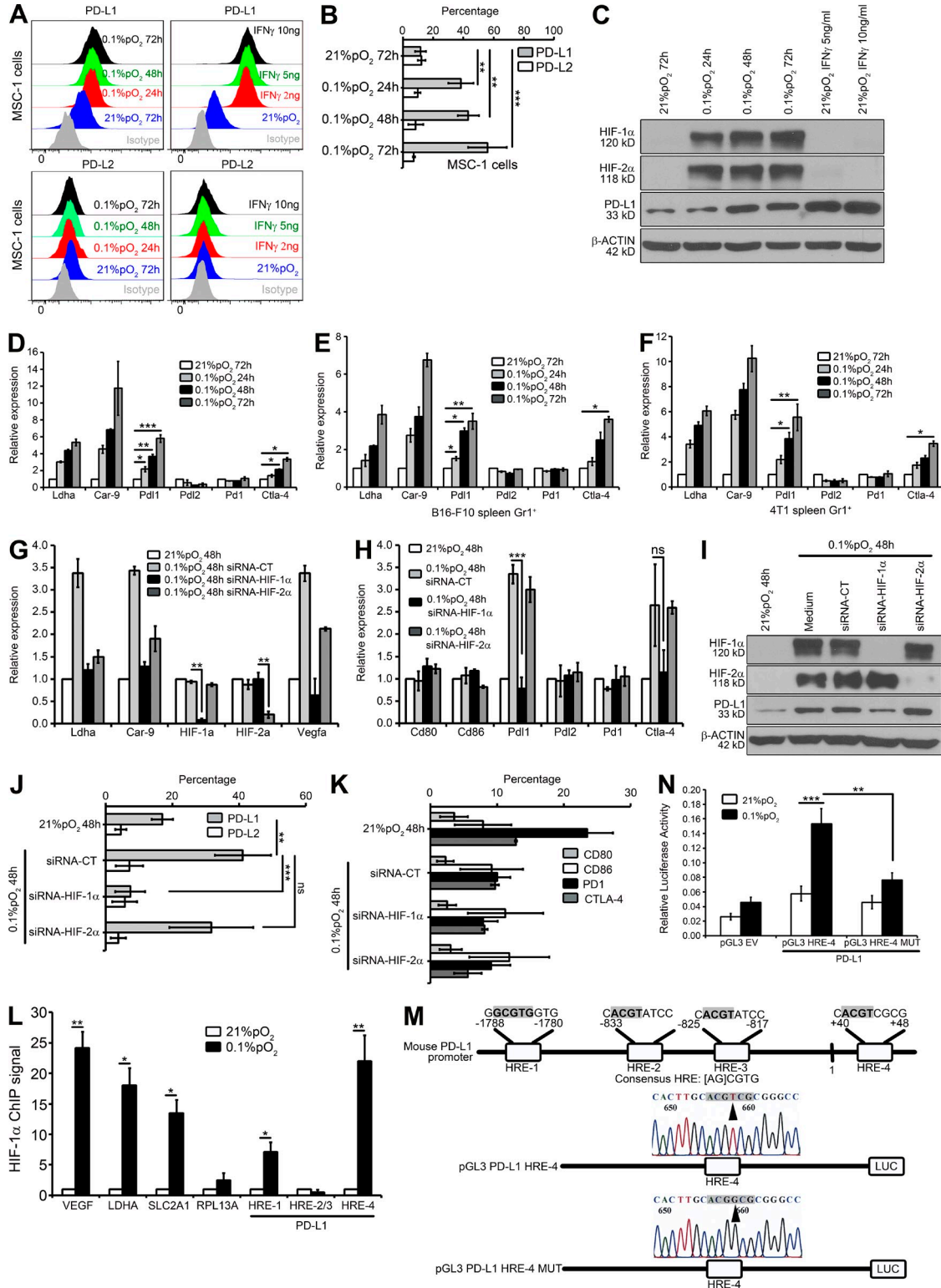
Figure 3. HIF-1 \alpha binds directly to the HRE in the PD-L1 proximal promoter and up-regulates its expression under hypoxia. (A–F) Surface expression levels of PD-L1 and PD-L2 (A and B) on MSC-1 cells cultured under normoxia and hypoxia (0.1% pO 2 ) at indicated times as compared with isotype control (gray-shaded histogram). IFN- \gamma was used as a positive control for PD-L1 up-regulation. Statistically significant differences (indicated by asterisks) between MSC-1 cells cultured under normoxia or hypoxia are shown (**, P < 0.005 ; ***, P < 0.0005 ). Three separate experiments with the same results were performed. Error bars indicate SD. (C) Western blot was performed to show HIF-1 \alpha , HIF-2 \alpha , and PD-L1 protein levels. \beta -Actin was used as a control. Three separate experiments with the same results were performed. (D–F) SYBR Green RT-qPCR was used to monitor Ldha, Car-9, Pd1, Pd2, Pd1, and Ctla-4 expression levels in B16-F10 spleen Gr1 + cells and 4T1 spleen Gr1 + cells. (G–I) SYBR Green RT-qPCR was used to monitor Ldha, Car-9, HIF-1 \alpha , HIF-2 \alpha , and Vegfa expression levels in 4T1 spleen Gr1 + cells and HIF-1 \alpha , HIF-2 \alpha , PD-L1, and \beta -ACTIN protein levels in MSC-1 cells under 0.1% pO 2 48h with various siRNA treatments. (J–L) Flow cytometry and ChIP analysis were used to monitor PD-L1 surface expression and HIF-1 \alpha ChIP signal in MSC-1 cells under different hypoxia and siRNA treatments. (M) Schematic of the mouse PD-L1 promoter with HRE-1 to HRE-4 sites and luciferase reporter constructs (pGL3 PD-L1 HRE-4 and pGL3 PD-L1 HRE-4 MUT).
