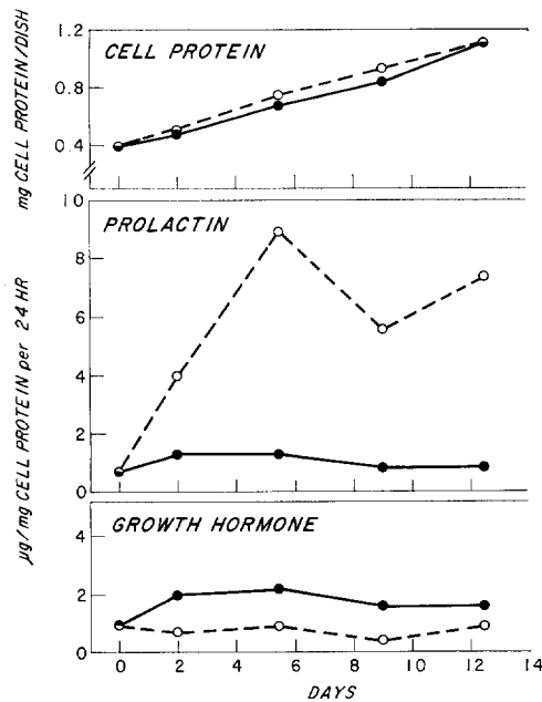
FIGURE 7 Effects of bovine hypothalamic extract on cell protein, and on prolactin and GH production by cultures of GH 3 cells. Duplicate dishes were used for each point. At zero time, medium either containing hypothalamic extract (0.14 ml extract/dish, 1.5 mg extract protein/dish) or lacking extract was added to each dish. Medium was collected at intervals from experimental (○) and control (●) dishes and was frozen for hormone assays. These dishes were washed and frozen for determination of cell protein. Medium containing hypothalamic extract did not fix C' with anti-prolactin or anti-GH, nor did it interfere with the assay of prolactin or GH in medium.
