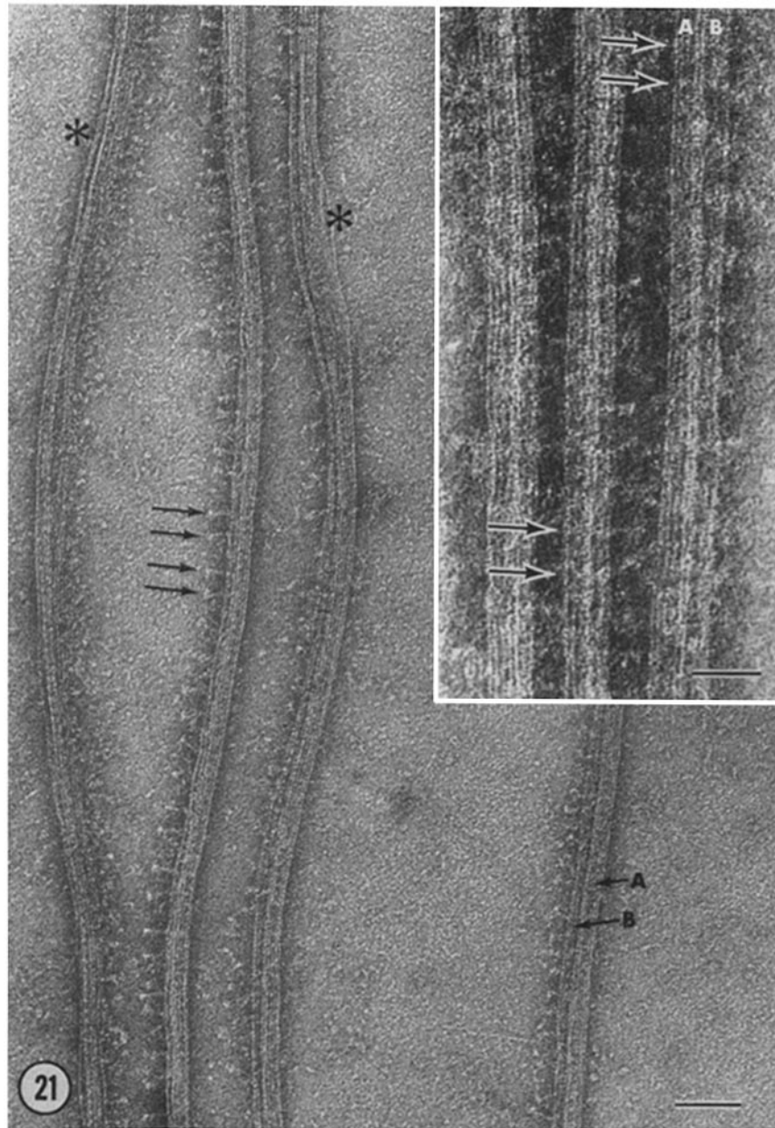
FIGURE 21 PTA negatively stained preparation showing four collapsed doublets with both A and B tubules visible. The radial links are often obscured, but are clear in regions (arrows). Along the doublets indicated by (*), the lack of links is due partially to doublet degradation. \times 96,000 . The insert illustrates three doublets with both A and B tubules clearly visible. The links lie transversely superimposed over each doublet (arrows) and project about 100 A past the lateral edge of the B tubule. The calibration bar represents 500 A. \times 200,000 .
